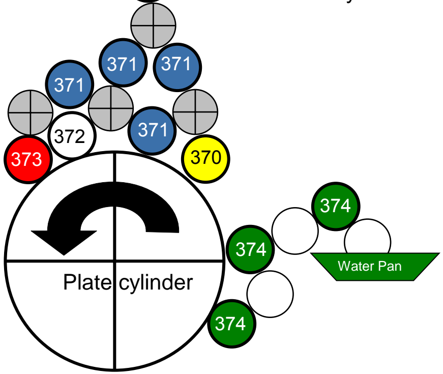
Conventional Water System
